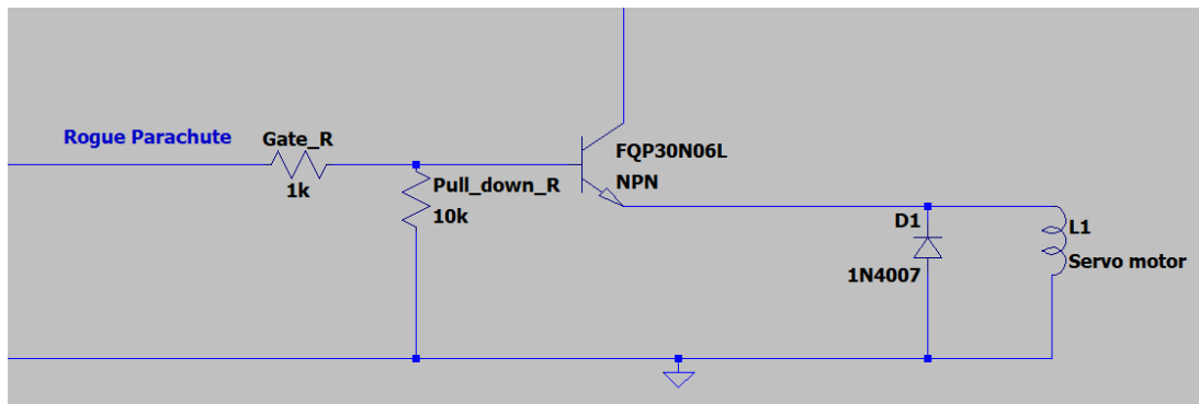
Figure 4: Droge parachute electrical diagram
