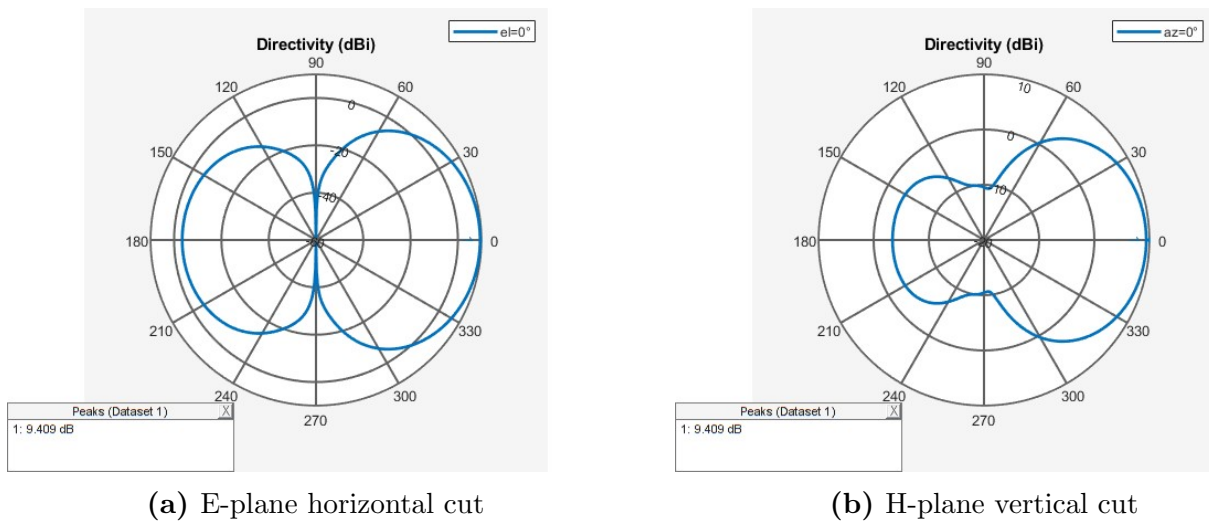
Figure 12: Radiation pattern plane cuts
