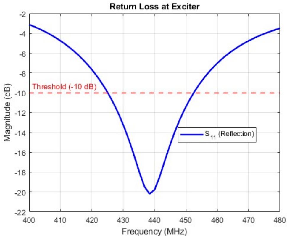
Figure 13: Simulated return loss ( S_{11} ) of the antenna
