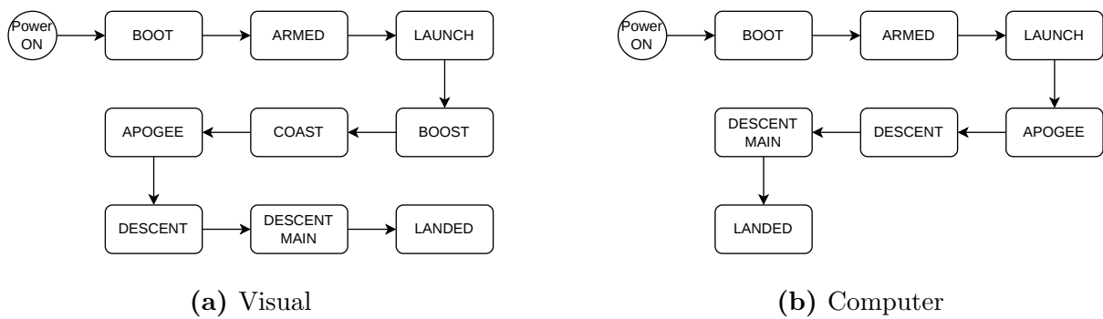
Figure 8: SRAD state diagrams
